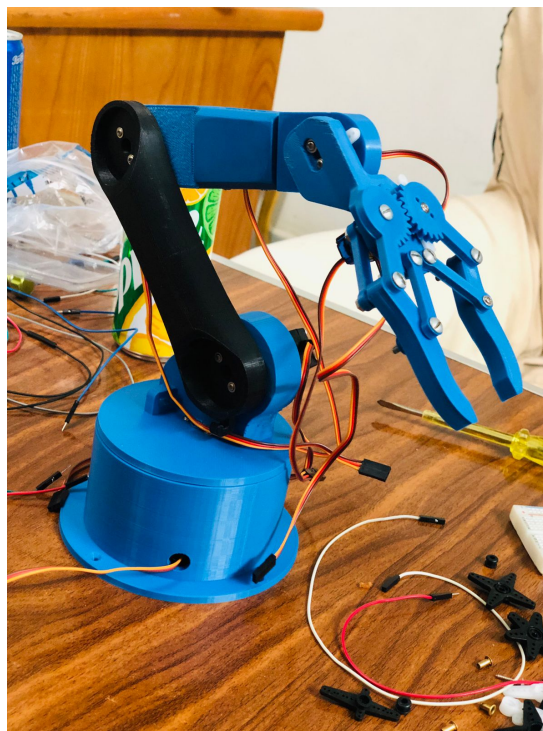
Figure 4.1: 3D printed Robotic Arm
